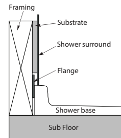
Flange Details: (U.S.)
