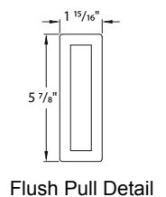
Flush Pull Detail
